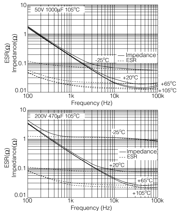
Fig. 1 - 11 Impedance, ESR vs. Frequency Characteristics
