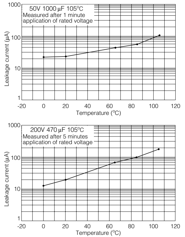
Fig. 1 - 12 Leakage current vs. Temperature Characteristic
