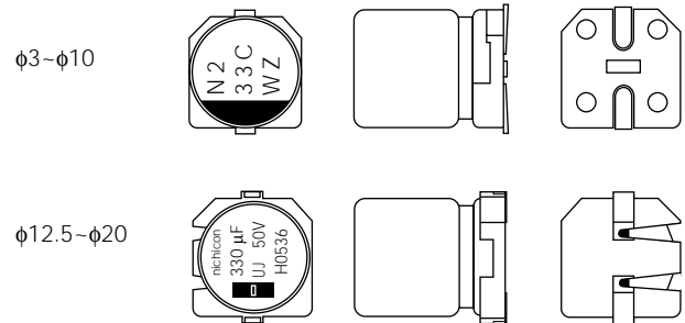
Fig. 2-23 Outward appearance of chip aluminum electrolytic capacitors
