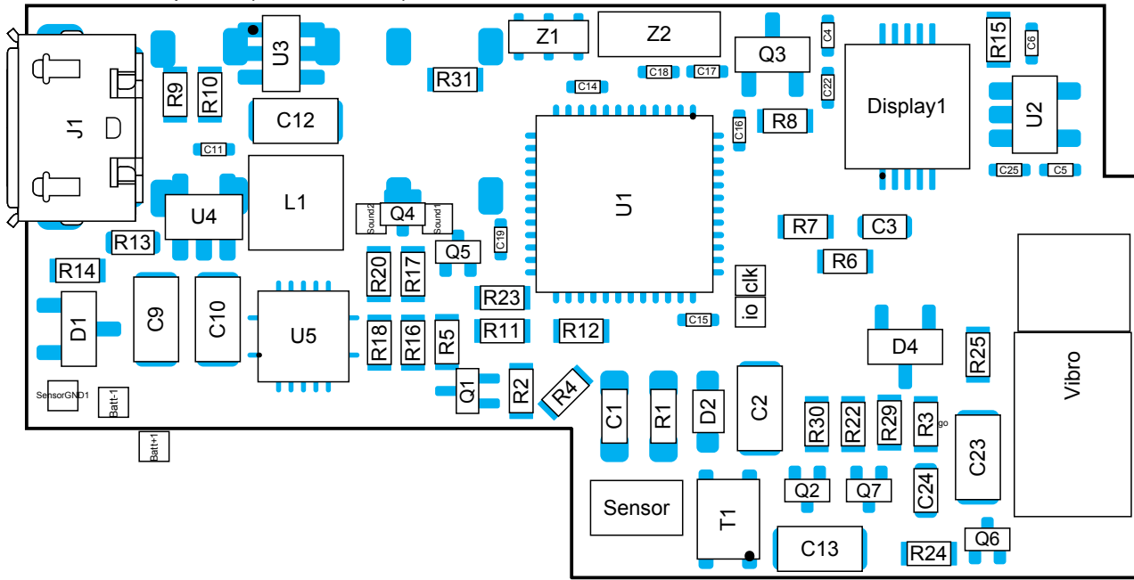
View from Top side (Scale 3.6914)
